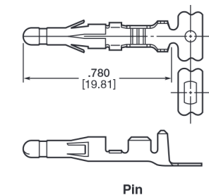
Pin
