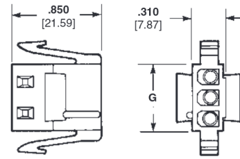
Socket Housing (Plug)
