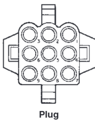
Plug
