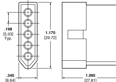
Plug (Free-Hanging)
