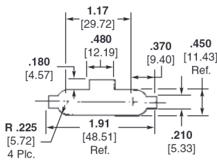
Panel Mount Cutout
