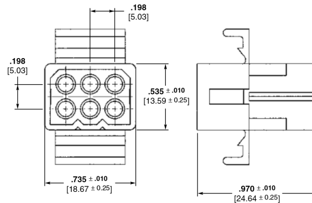
Plug
