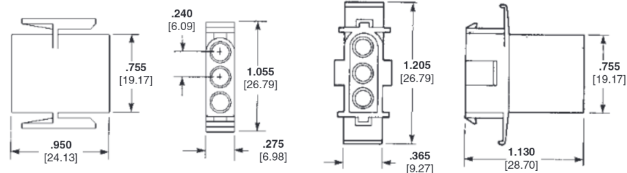
Socket Housing (Plug) Part No. 1-350346-0
